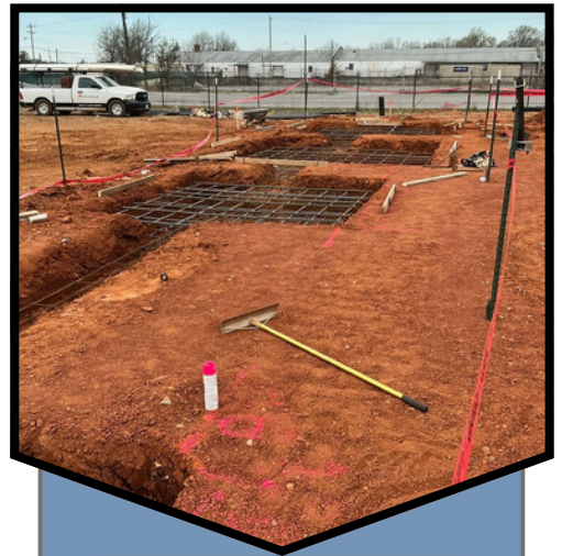
Footings
